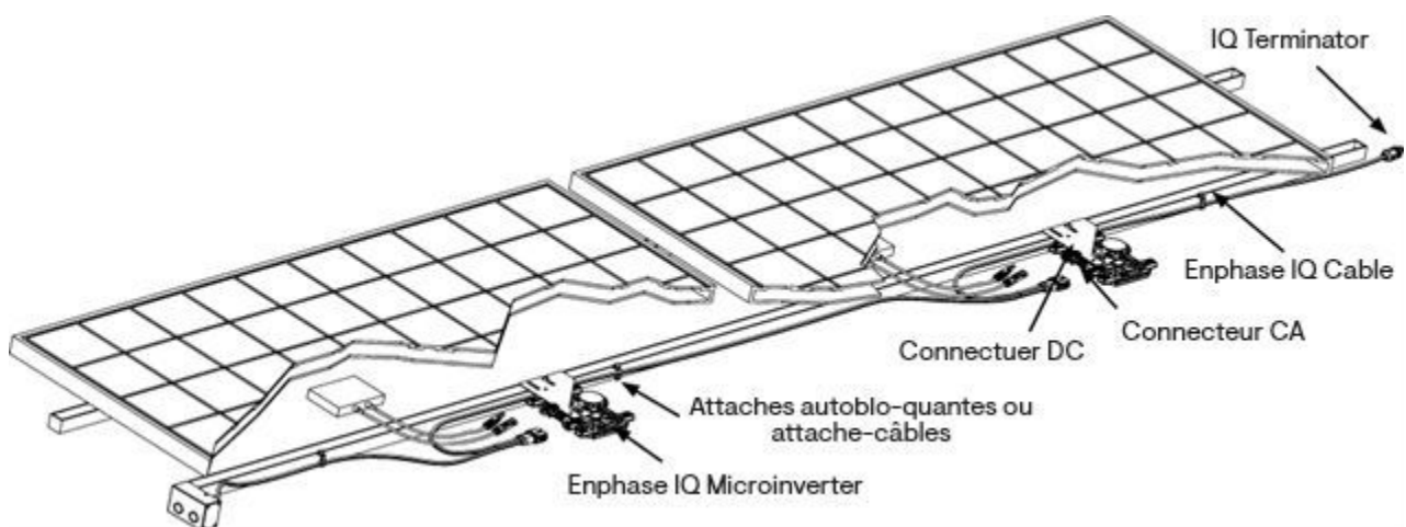
Illustration 1: Montage horizontal
